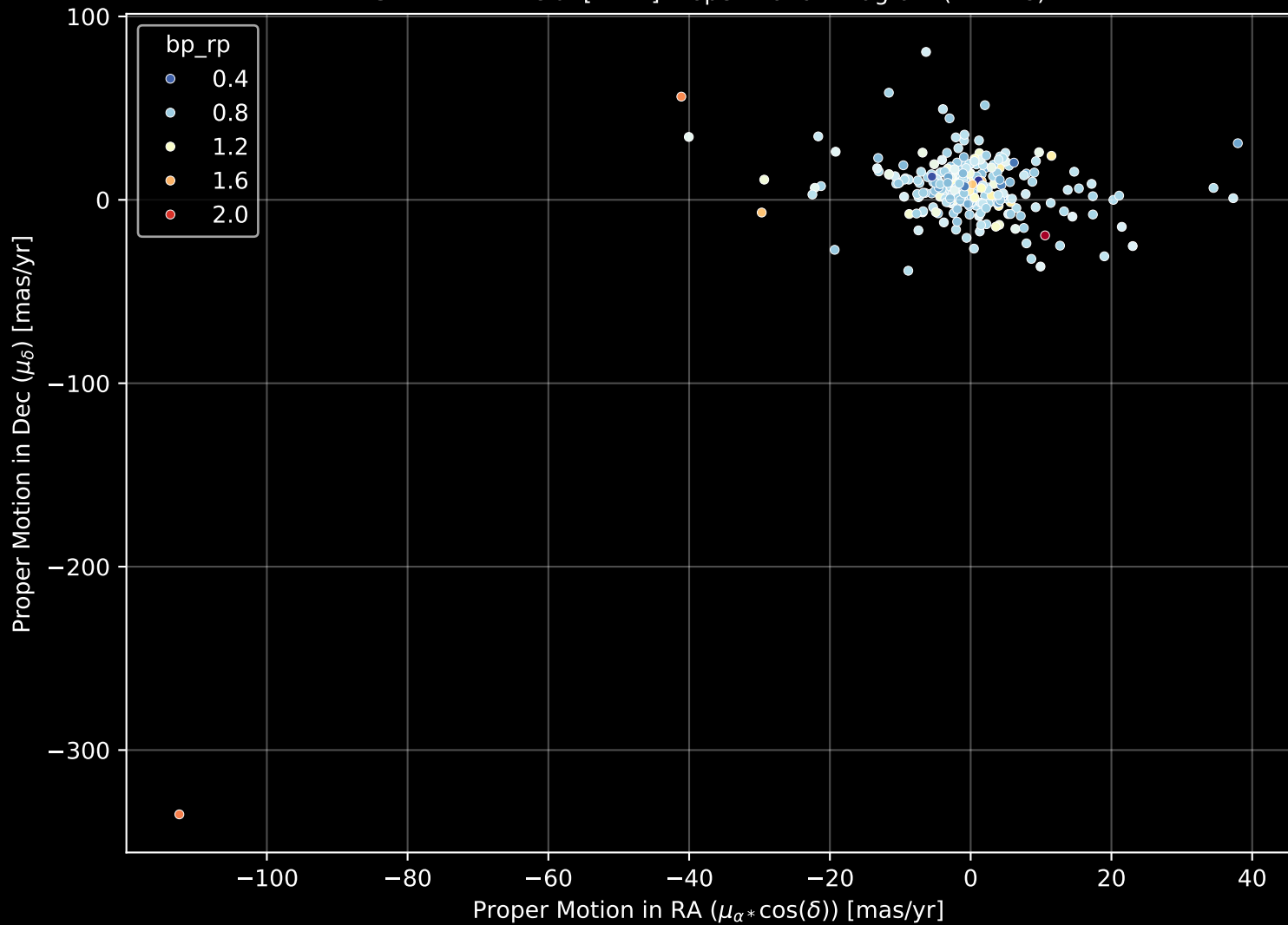
GALAH DR4 Field: [1277] Proper Motion Diagram (n= 278)
