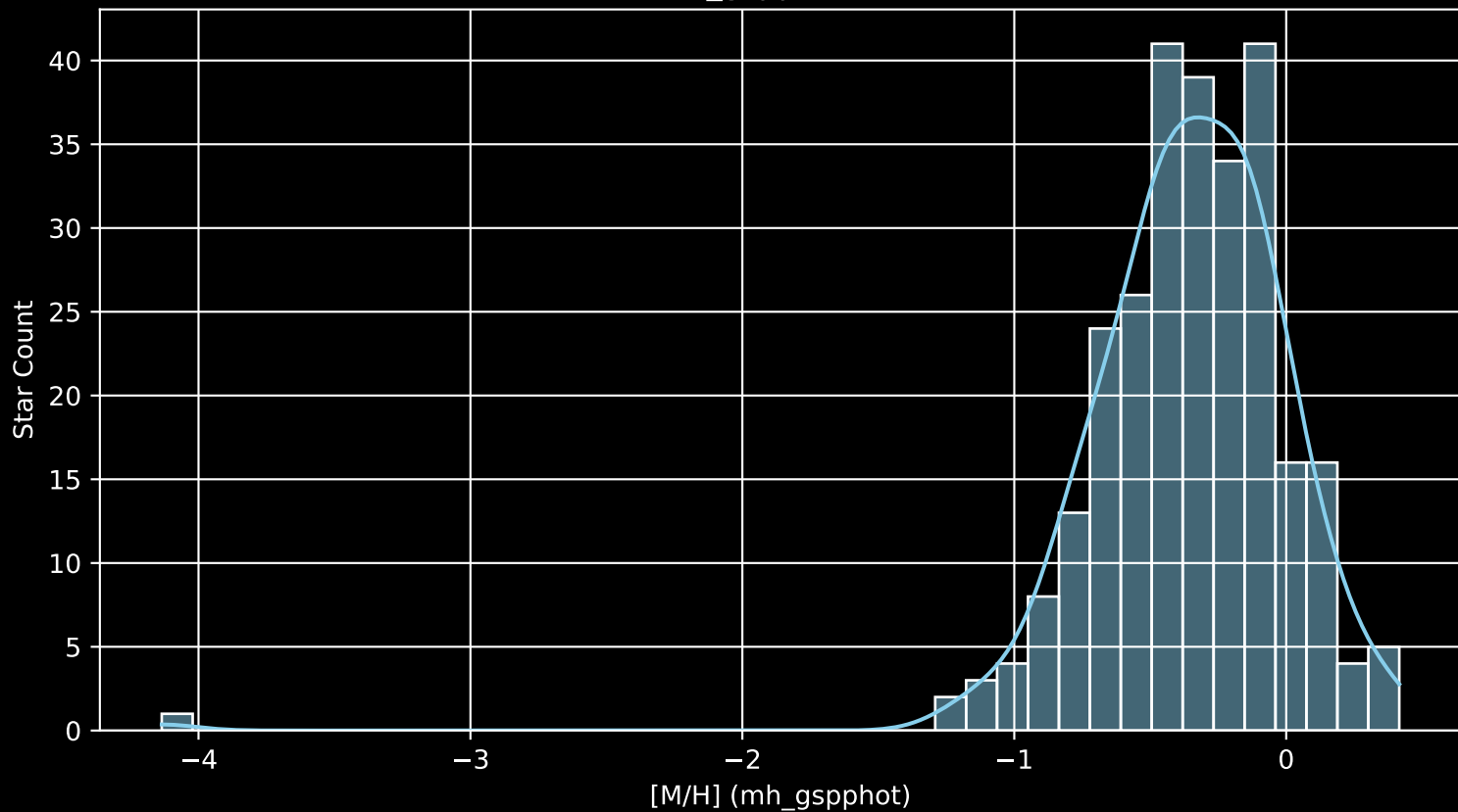
GALAH DR4 Field: [1277] [M/H] (mh_gspphot) (n= 277)
