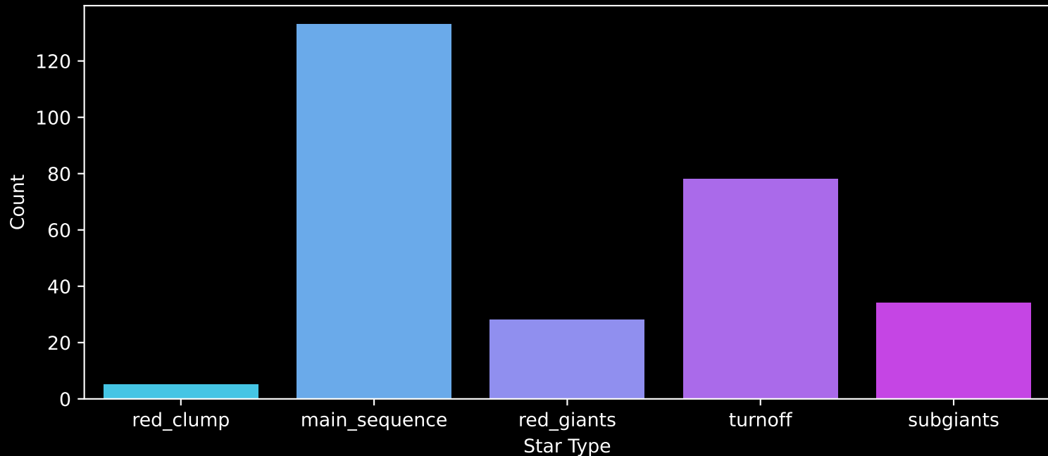
GALAH DR4 Field: [1277] Count plot of Star Type
