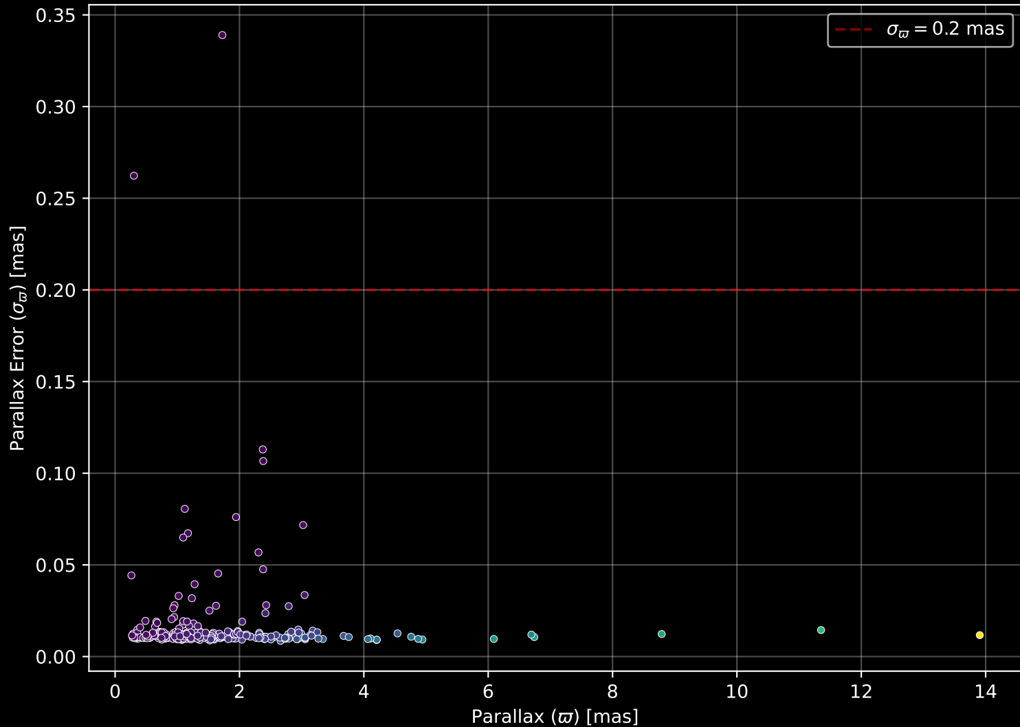
GALAH DR4 Field: [1277] Parallax Quality (n= 278)
