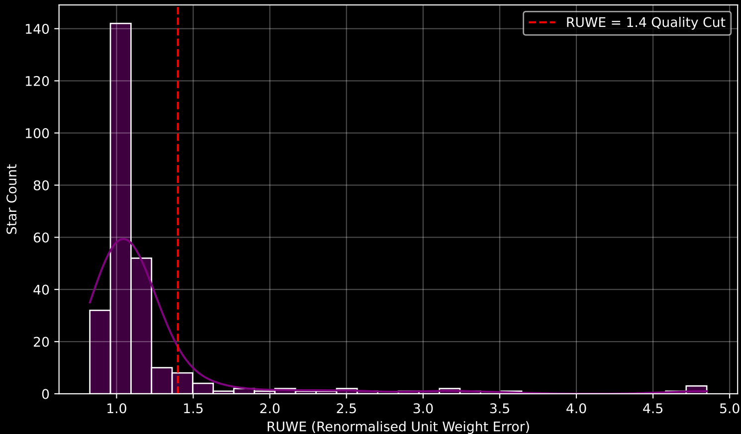
GALAH DR4 Field [1277] RUWE Distribution (n= 269)
